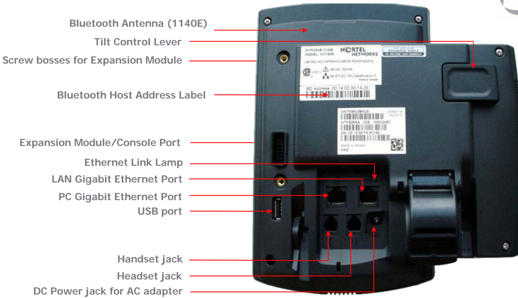
Back features – stand removed for clarity
